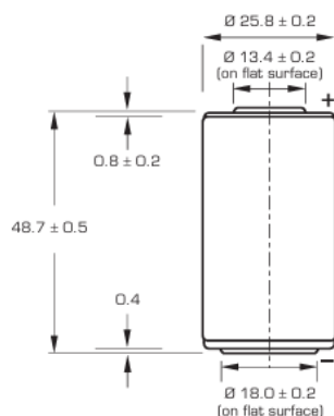
Finished version with flat positive end cap
