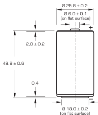
Finished version with protruding positive end cap
